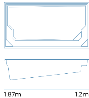
8m Diamond Pool
