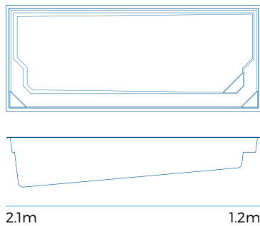
11m Diamond Pool
