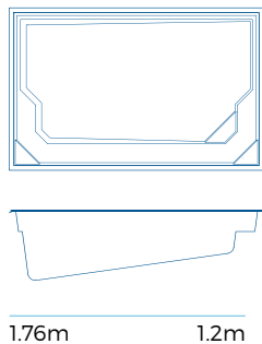
7m Diamond Pool
