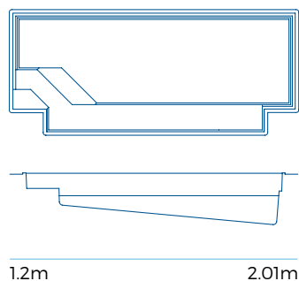
10m Sapphire Pool
